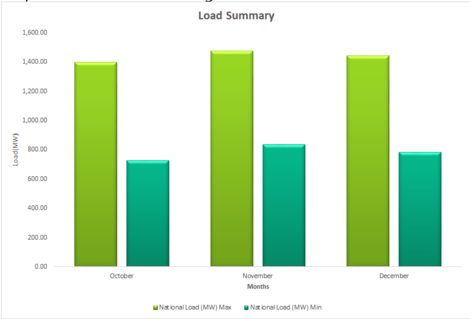
Graph 4.1 National Load using method- 1
