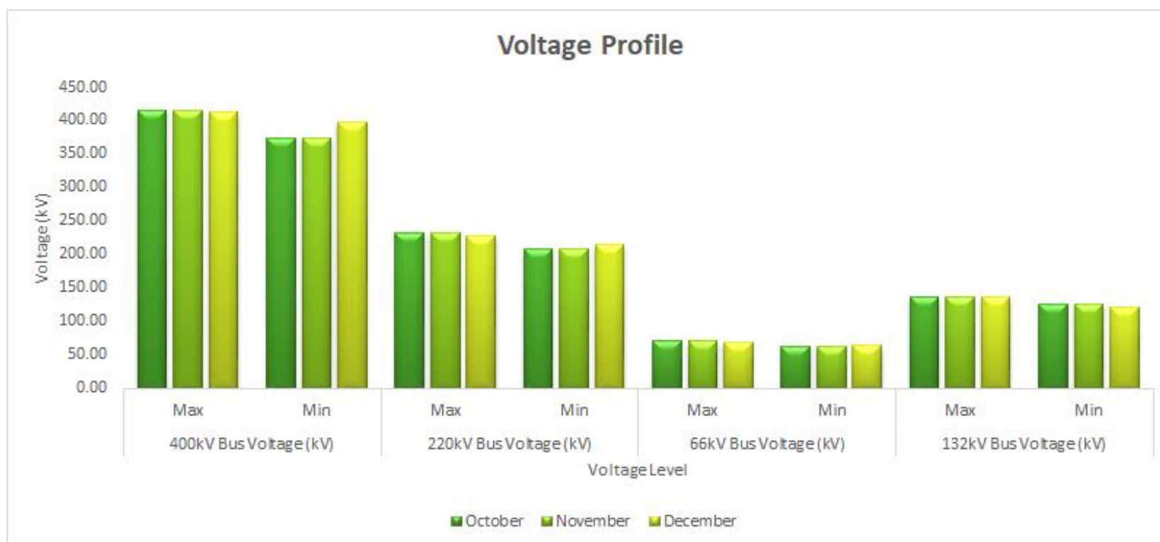
Graph 9.1 Voltage Summary for the month of October to December 2025
