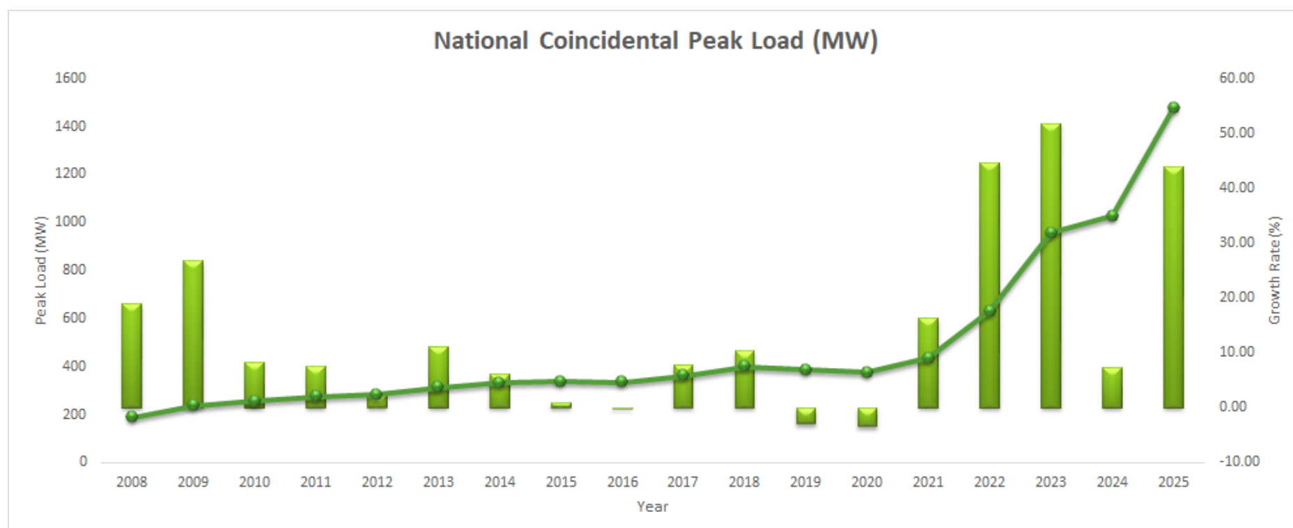
Graph 3.1. The growth in National Peak Demand since 2008
