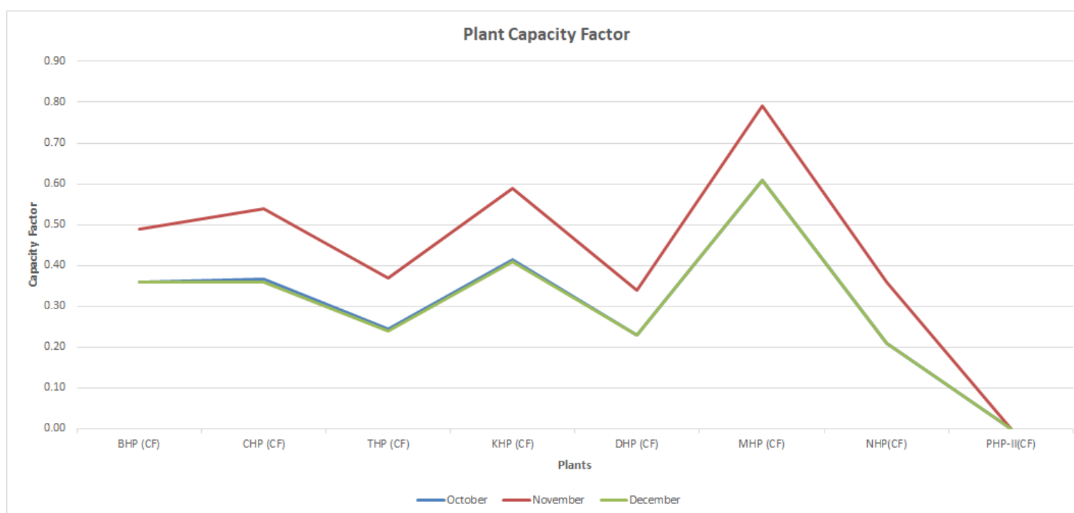
Graph 6.2. Capacity factor of various hydropower plants
