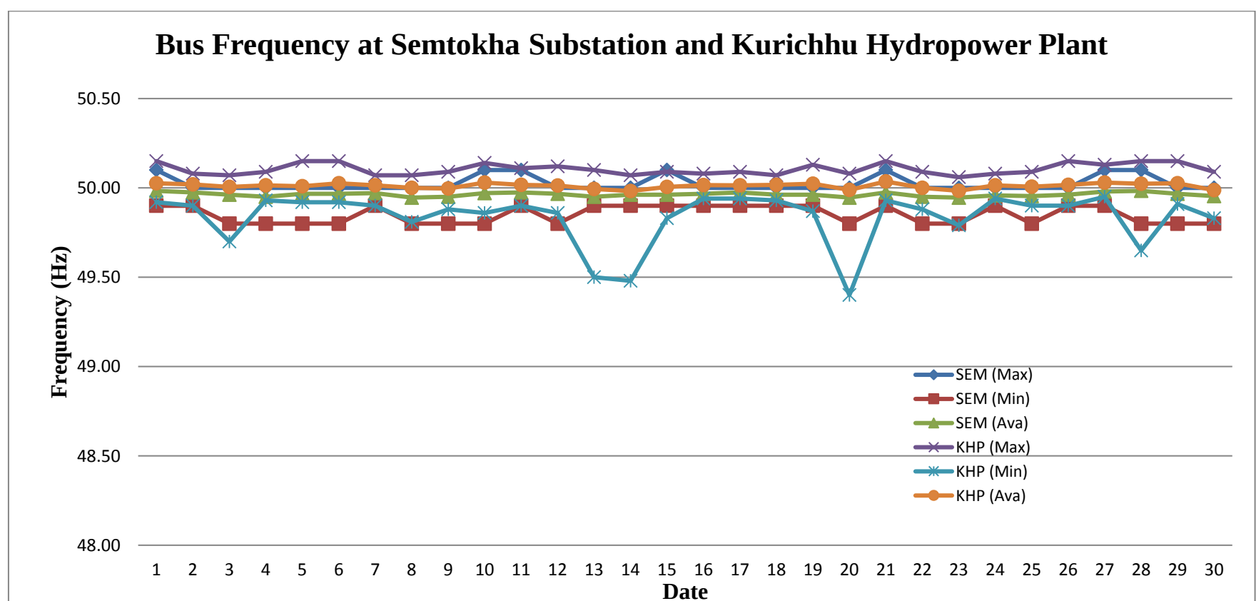
Graph: Daily maximum, minimum and average frequency for the month of May, 2020
