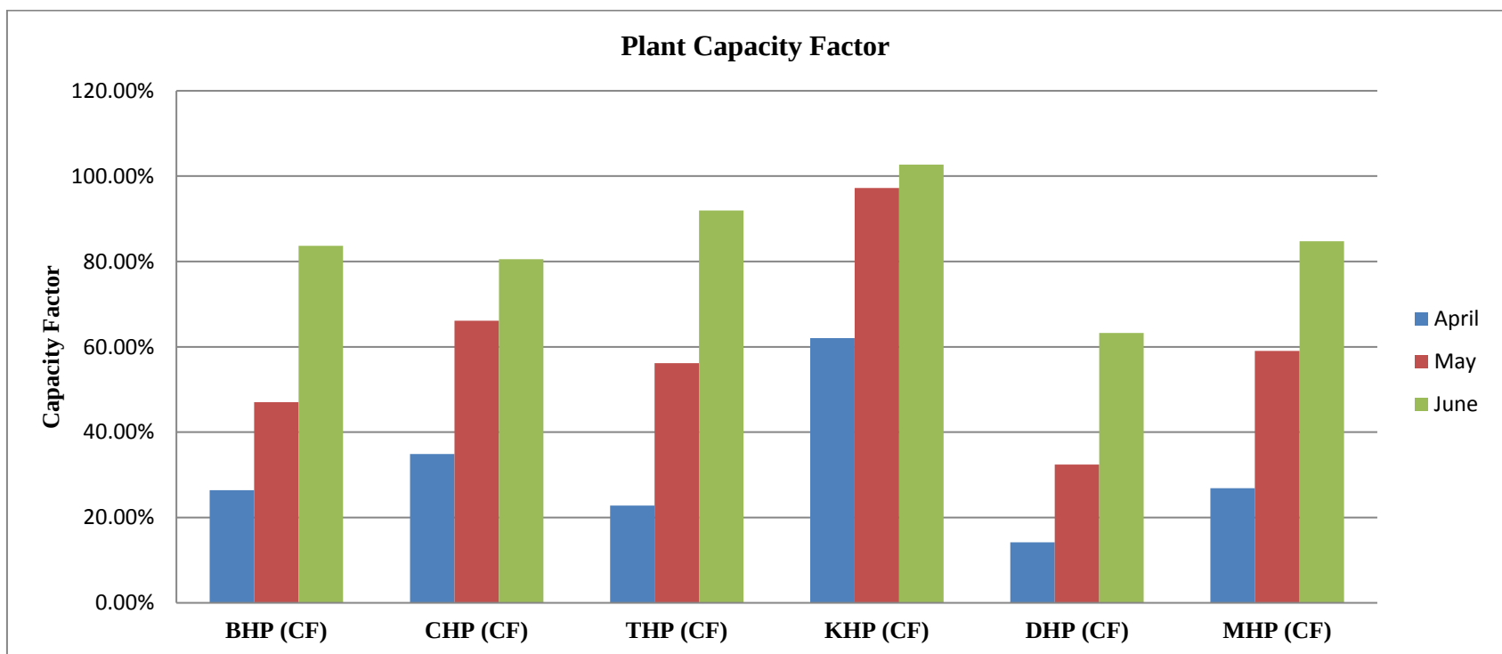
Graph 4.2.1: Capacity factor of various hydropower plants
