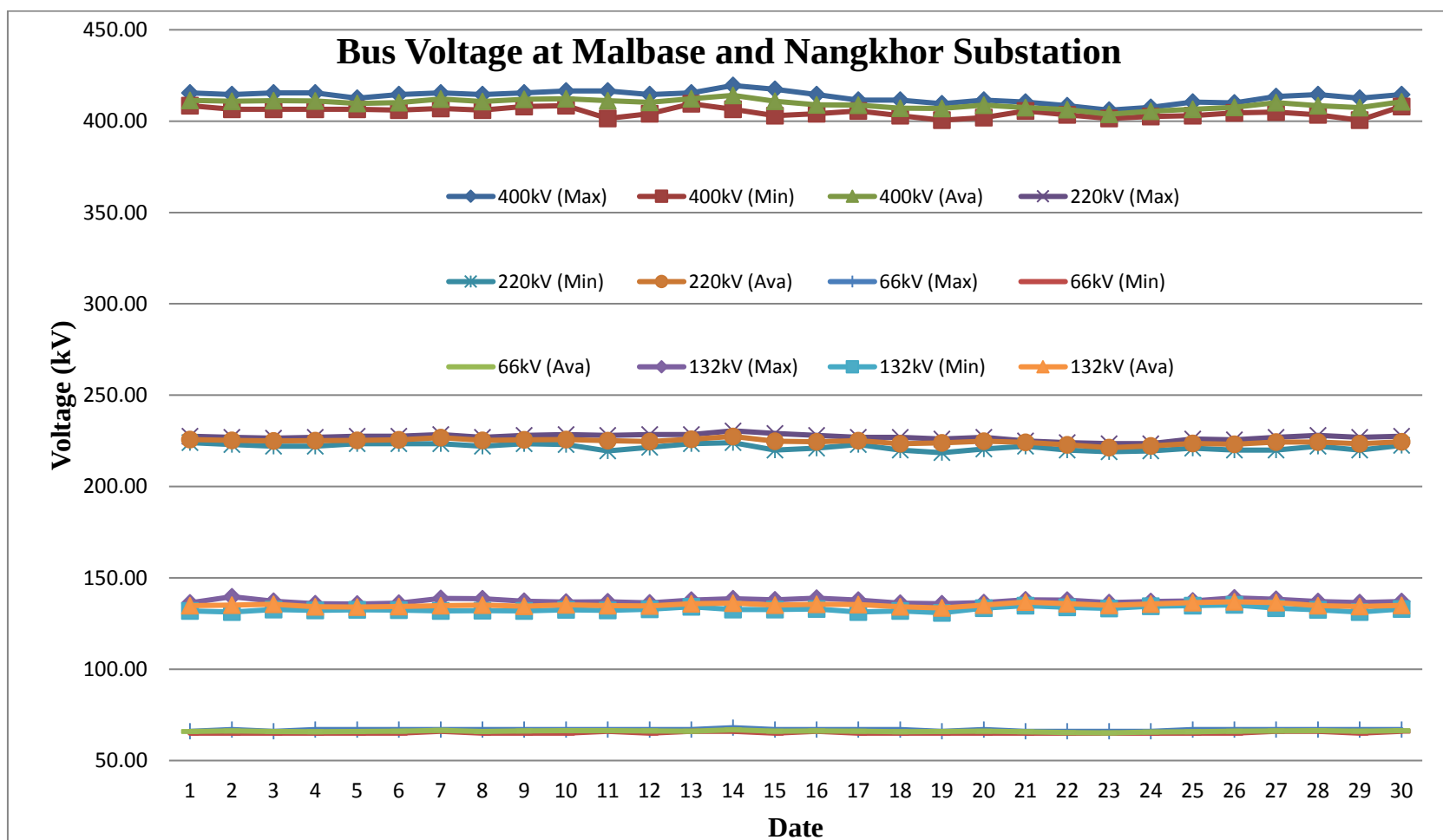
Graph: Daily maximum, minimum and average Voltage for the month of May, 2020
