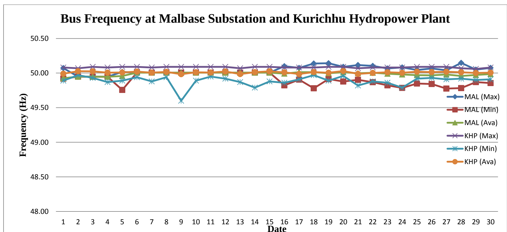
Graph: Daily maximum, minimum and average frequency for the month of April, 2020
