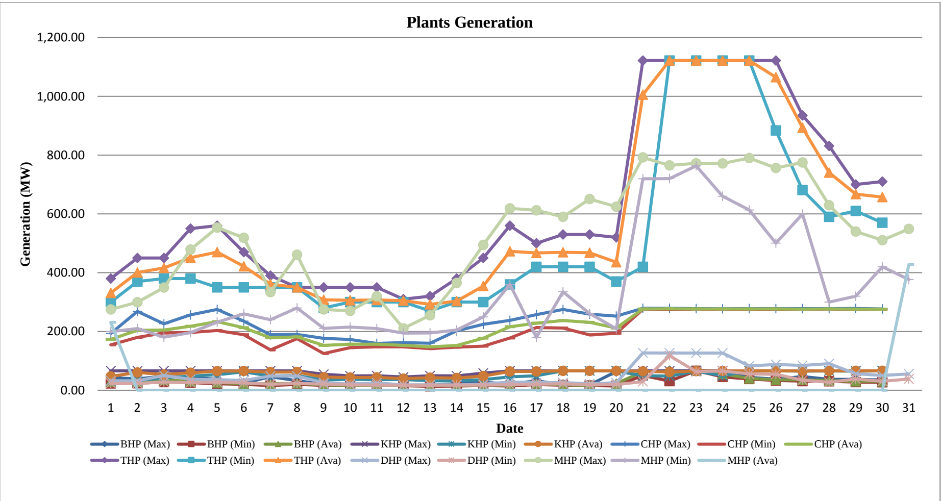
Graph: Generation for the month of May, 2020
