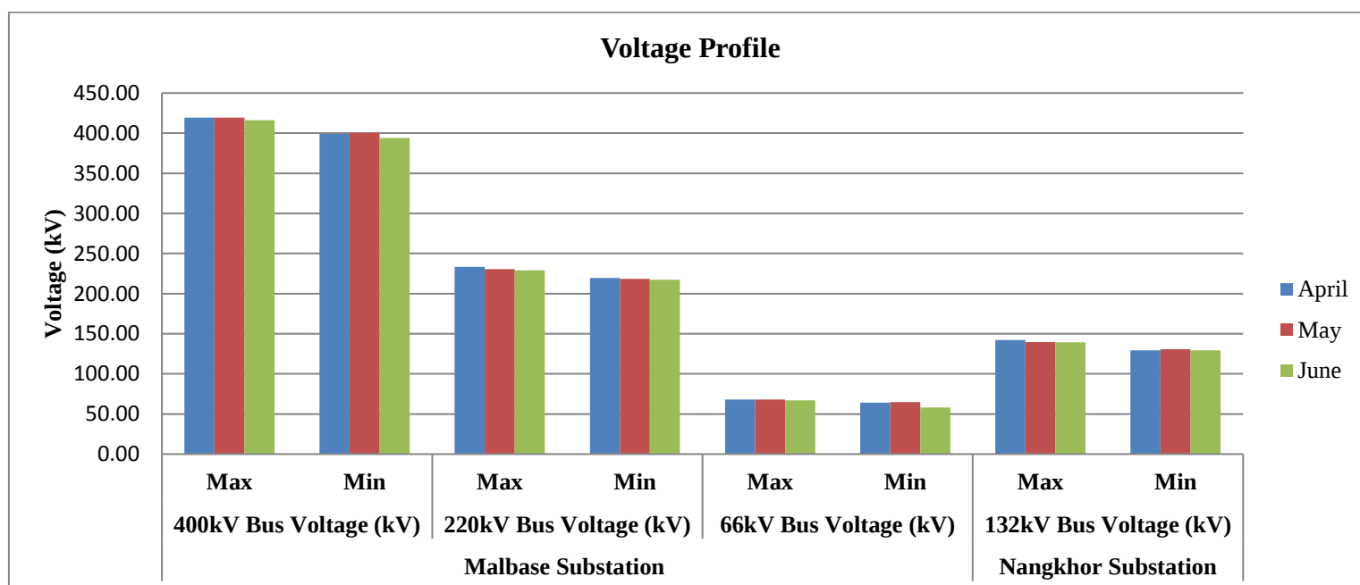
Graph 7.4.1. Voltage Summary for the month of April to June, 2020
