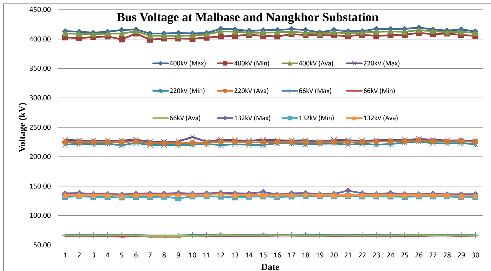
Graph: Daily maximum, minimum and average Voltage for the month of April, 2020
