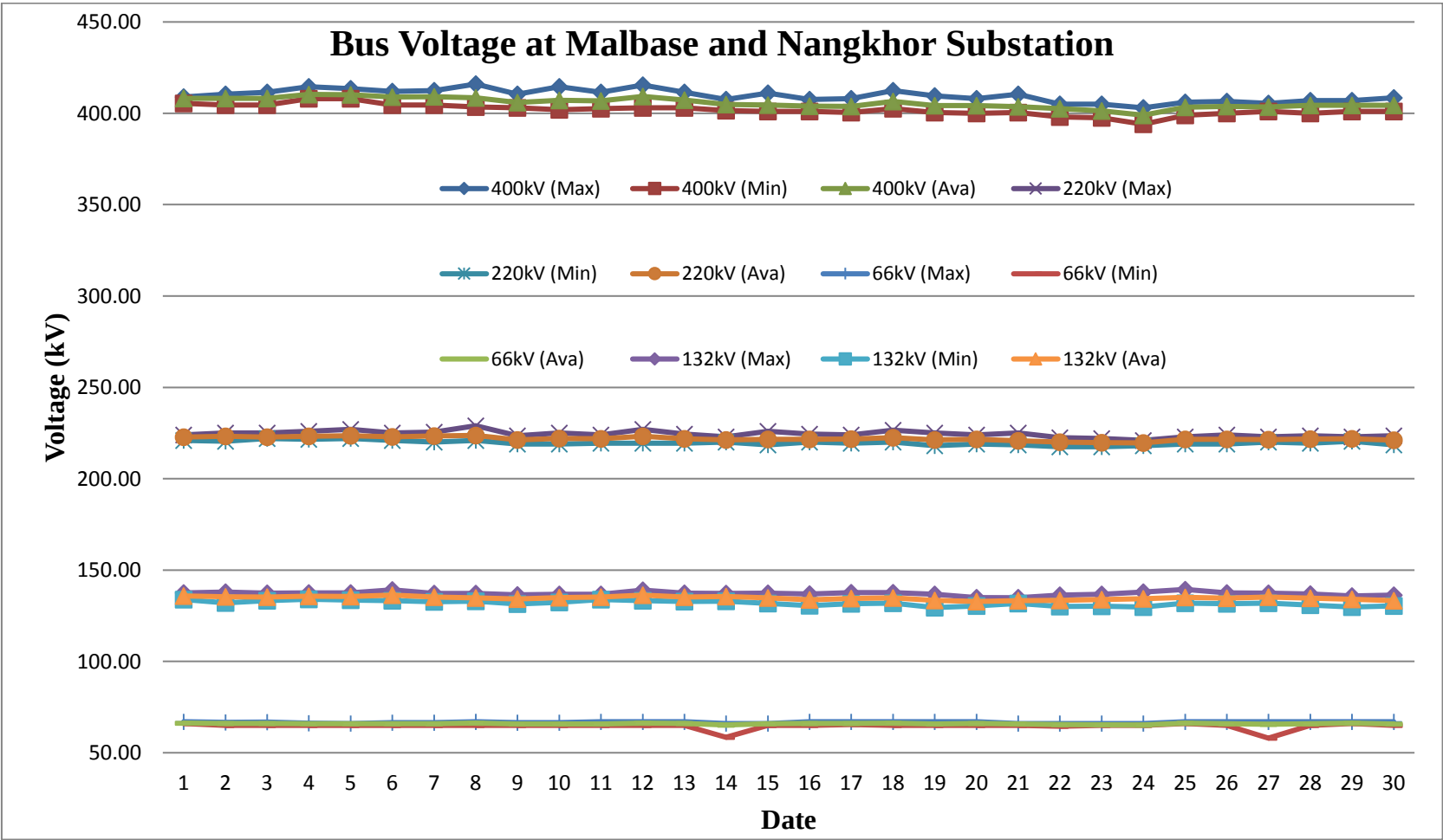
Graph: Daily maximum, minimum and average Voltage for the month of June, 2020
