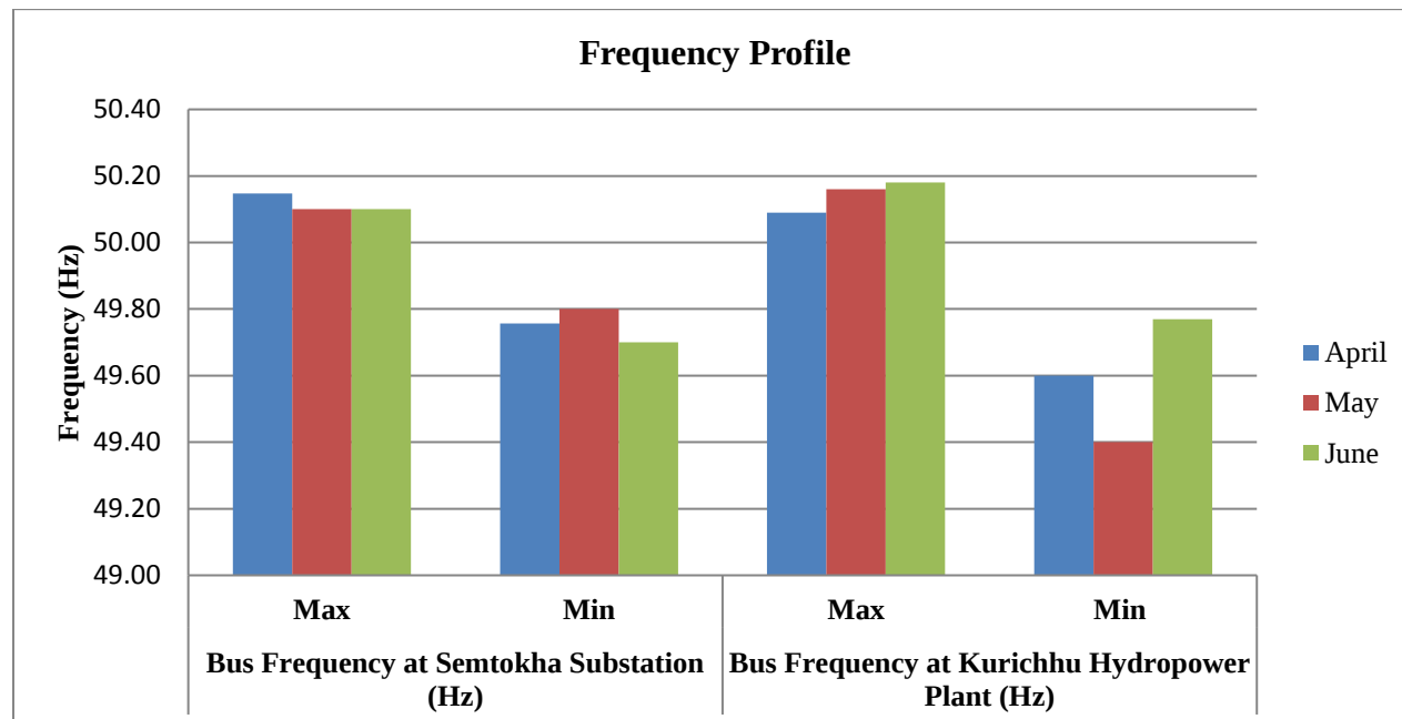
Graph 6.4.1. Frequency summary for the month of April to June, 2020
