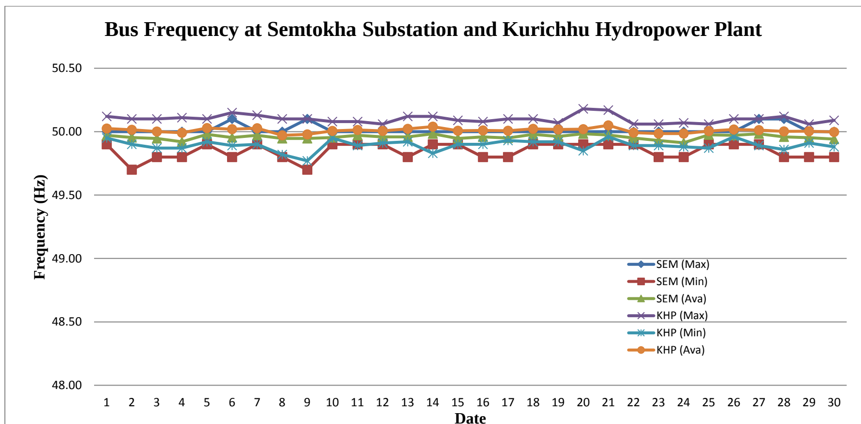
Graph: Daily maximum, minimum and average frequency for the month of June 2020
