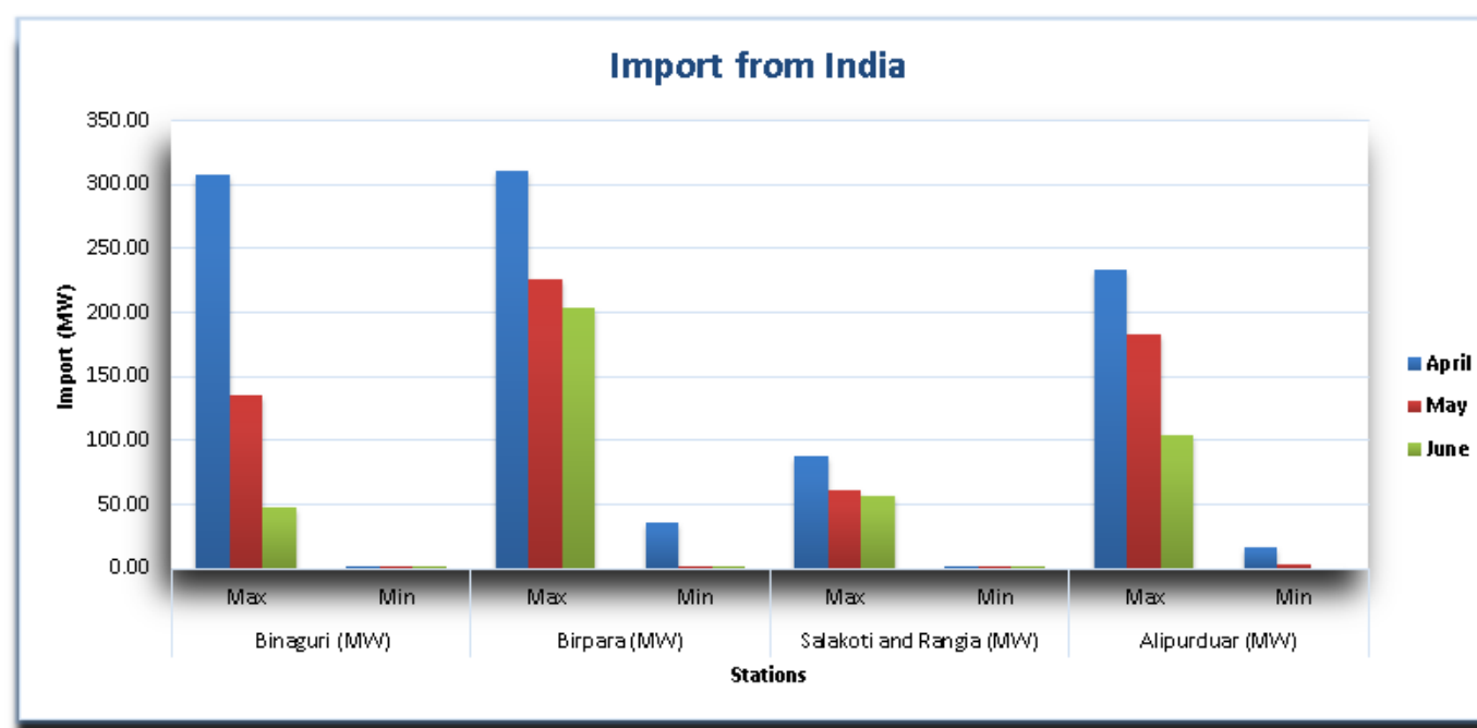
Graph 7.2. Import of electricity from India
