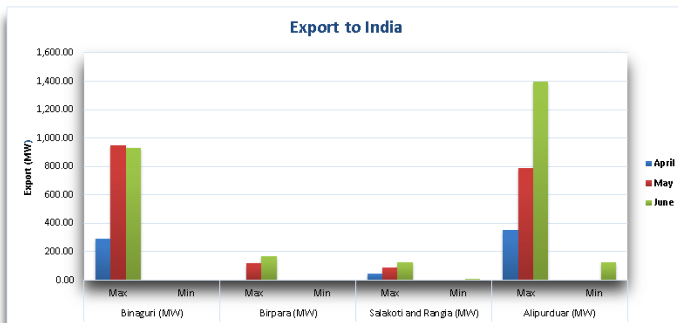
Graph 7.1. Export of electricity to India
