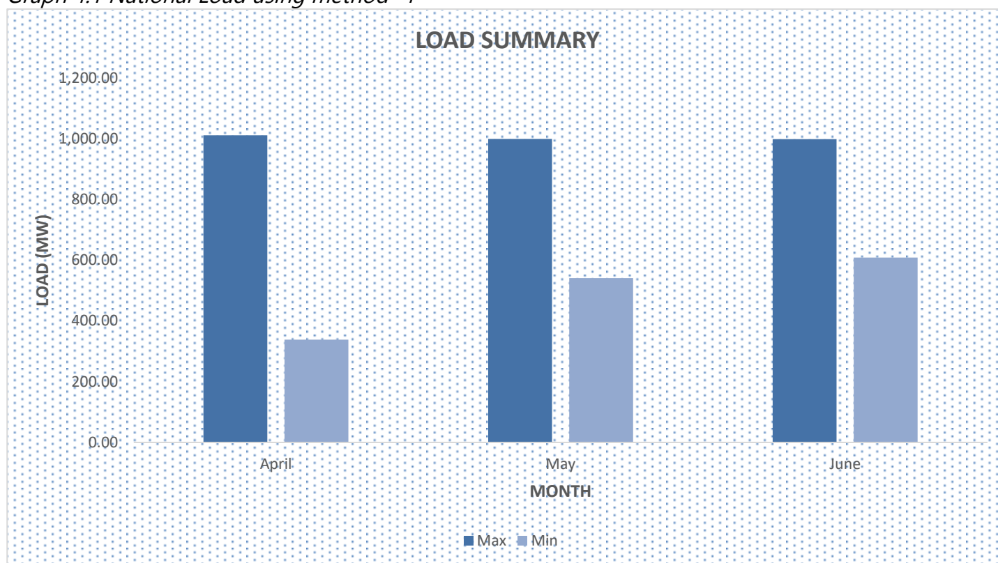
Graph 4.1 National Load using method- 1
